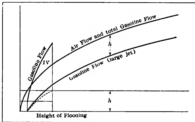
Fig. 7—Curves taken from tests made with a Zenith carburetor
